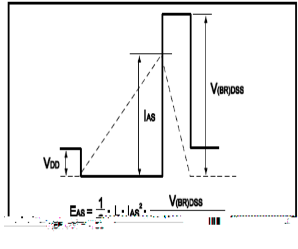
Fig.12 Avalanche Waveform
