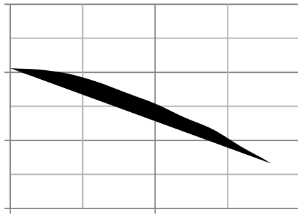
Fig.3 Threshold Voltage V.S Junction Temperature
